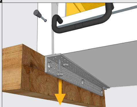
24. Remove the 8 hex bolts M10x30 under the oven and keep them
