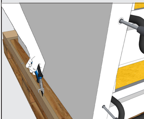
17. Remove the staples from one side of the oven
